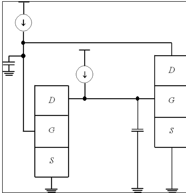
Fig 1a: Structure of the considered filter [19]
