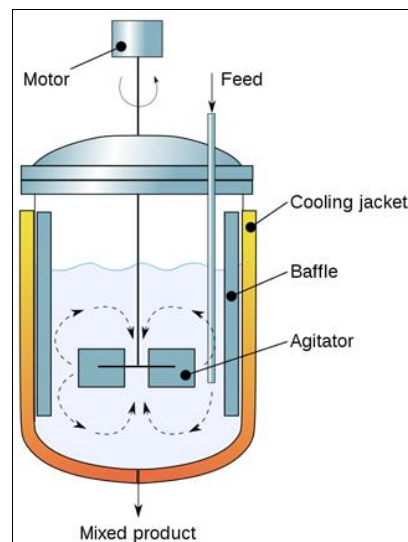
Fig 1: An isometric view of the batch plastic mixer
